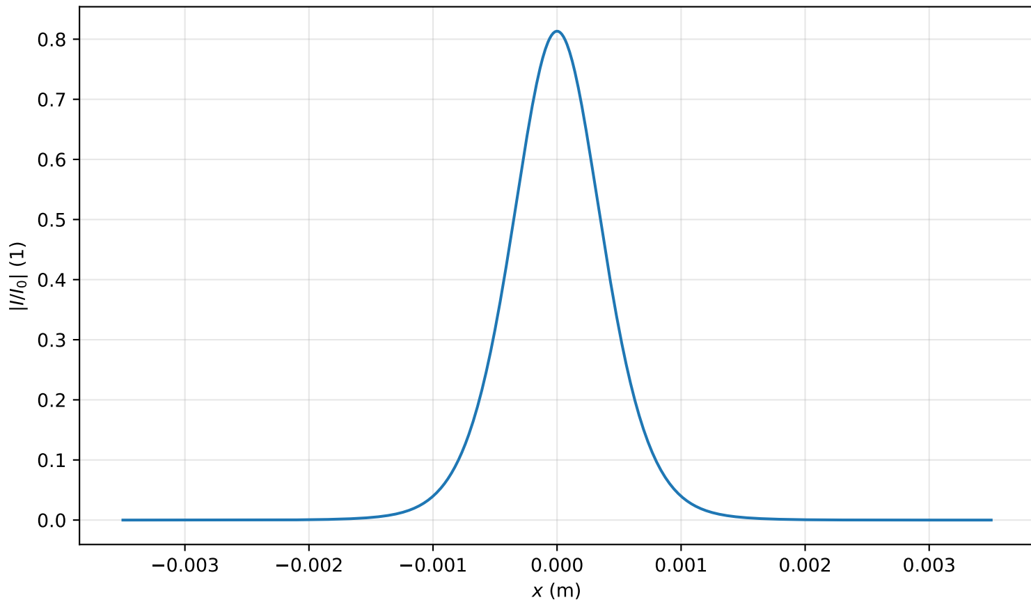
Intensity profile I(x, y = 0, z = 2.468m)/I_0 , P_{in}=0.6P_{cr} , artificial time
